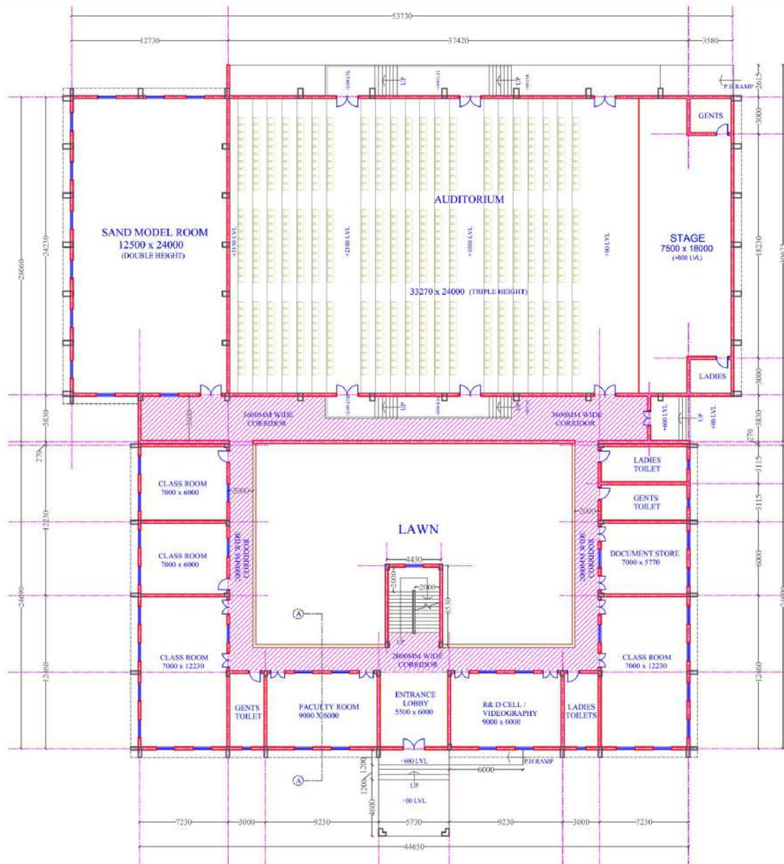
TRAINING BLOCK GROUND FLOOR PLAN PLINTH AREA 2200SQ.M
