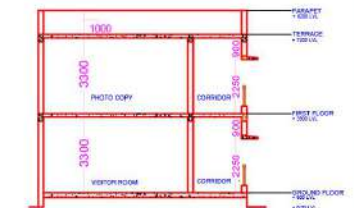
SECTION-XX'
