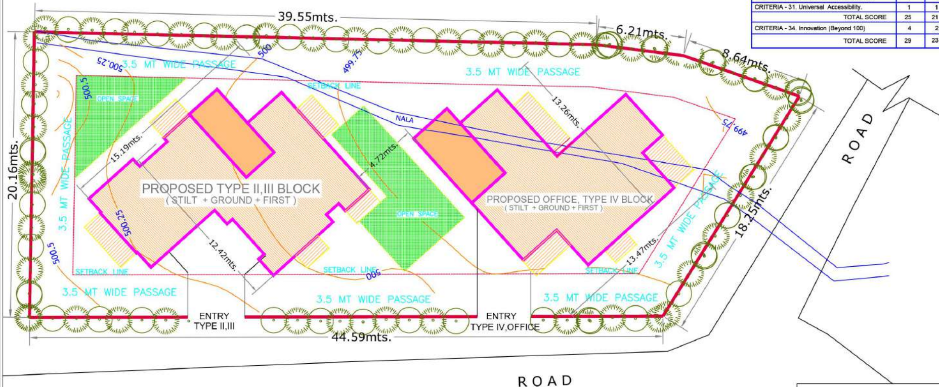
LAYOUT PLAN
