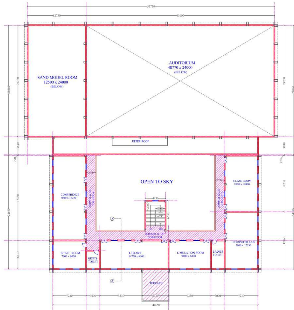
TRAINING BLOCK FIRST FLOOR PLAN PLINTH AREA 728SQ.M
