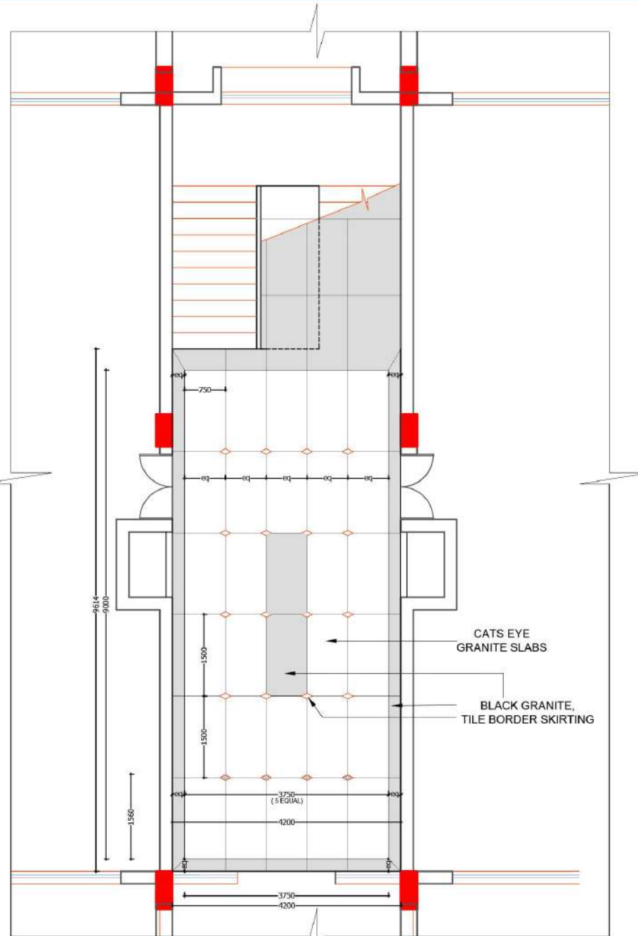
GROUND FLOOR MAIN ENTRY FLOORING PATTERN
